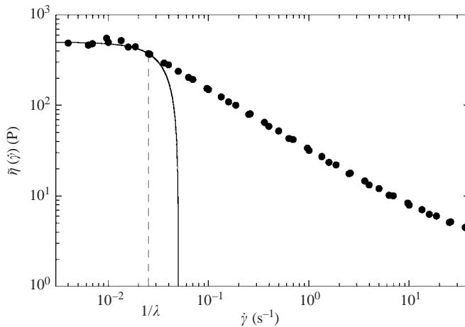
FIGURE 2. The apparent shear viscosity of the solution of 0.16% xanthan gum in 80:20 glycerol/water at 25 °C. An approximation of the relaxation time \lambda is obtained from the shear rate at which \tilde{\eta}(\dot{\gamma}) thins below \tilde{\eta}_0 (dashed line). The solid line corresponds to a theoretical fit with (3.5) as discussed in §3.2.
